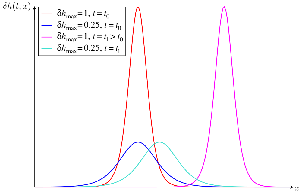
Figure V.2 – Profile of the soliton solution (V.45).
