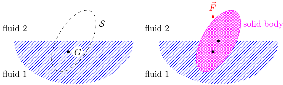
Figure IV.1 – Gedankenexperiment to illustrate Archimedes' principle.
