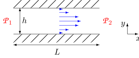
Figure VI.2 – Flow between two motionless plates for \mathcal{P}_1 > \mathcal{P}_2 , i.e. \Delta\mathcal{P} > 0 .
