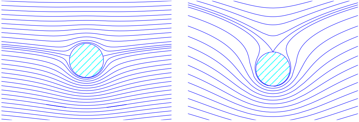
Figure IV.13 – Streamlines for the cyclic potential flow past a (rotating) cylinder (IV.50a) with \Gamma/(4\pi Rv_\infty) = 0.25 (left) or 1 (right).
