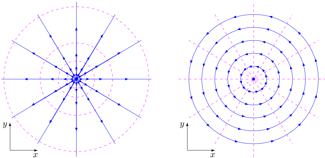
Figure IV.9 – Streamlines (full) and equipotential lines (dashed) for a flow source (IV.42c) (left) and a pointlike vortex (IV.43b) (right).
