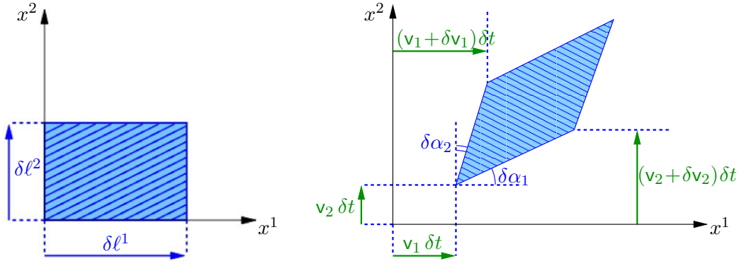
Figure II.2 – Evolution of a material rectangle caught in the motion of a continuous medium between times t (left) and t + \delta t (right).
