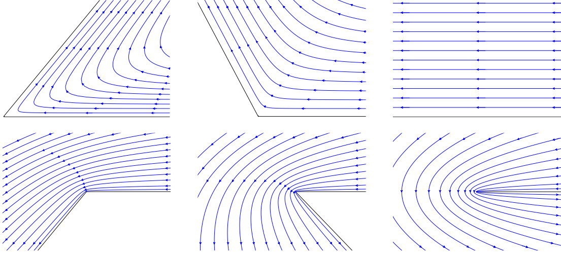
Figure IV.11 – Streamlines for the flow defined by potential (IV.47a) with from top to bottom and from left to right n = 3, \frac{3}{2}, 1, \frac{3}{4}, \frac{3}{5} and \frac{1}{2} .
