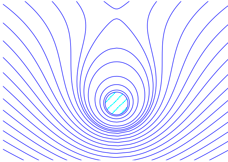
Figure IV.14 – Streamlines for the cyclic potential flow past a (rotating) cylinder (IV.50a) with \Gamma/(4\pi Rv_\infty) = 4 .
