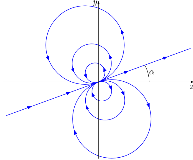
Figure IV.10 – Streamlines for a flow dipole (IV.44a) centered on the origin.
