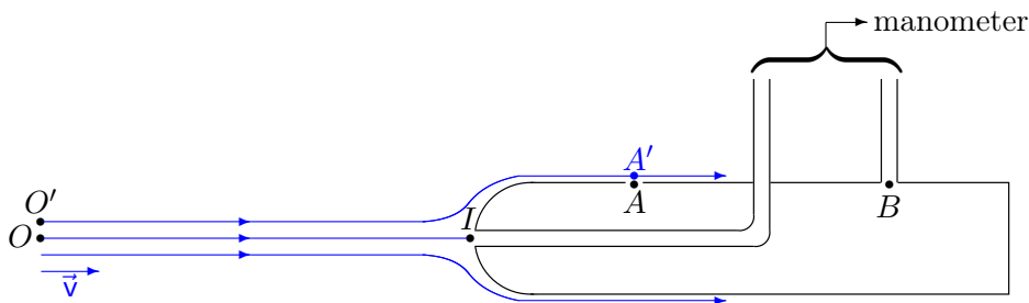
Figure IV.4 – Flow around a Pitot tube.
