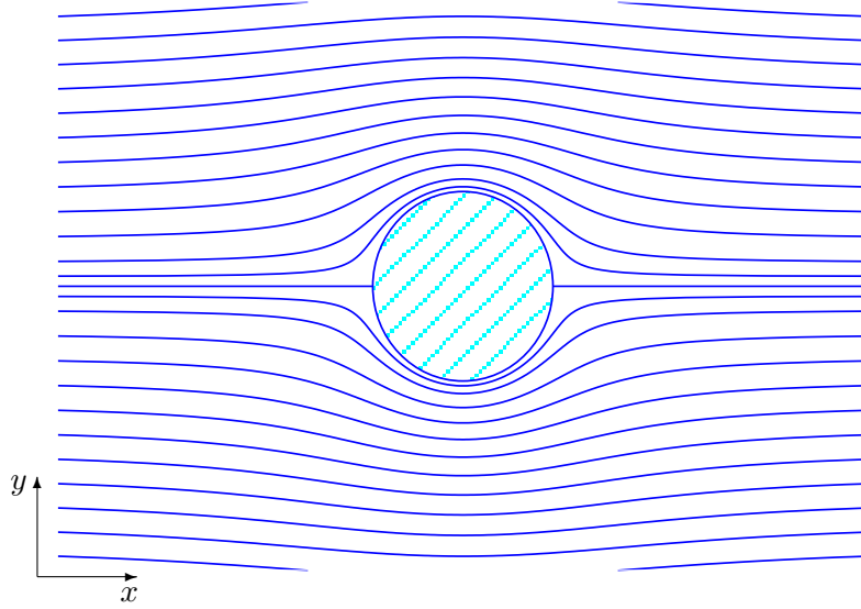
Figure IV.12 – Streamlines for the acyclic potential flow past a cylinder (IV.48a).
