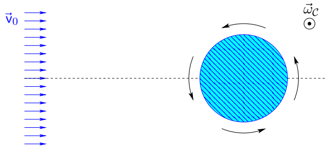
Figure IV.4 – Fluid flow around a rotating cylinder.
