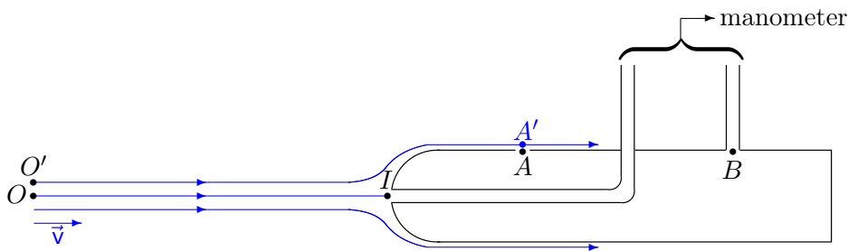
Figure IV.3 – Flow around a Pitot tube.
