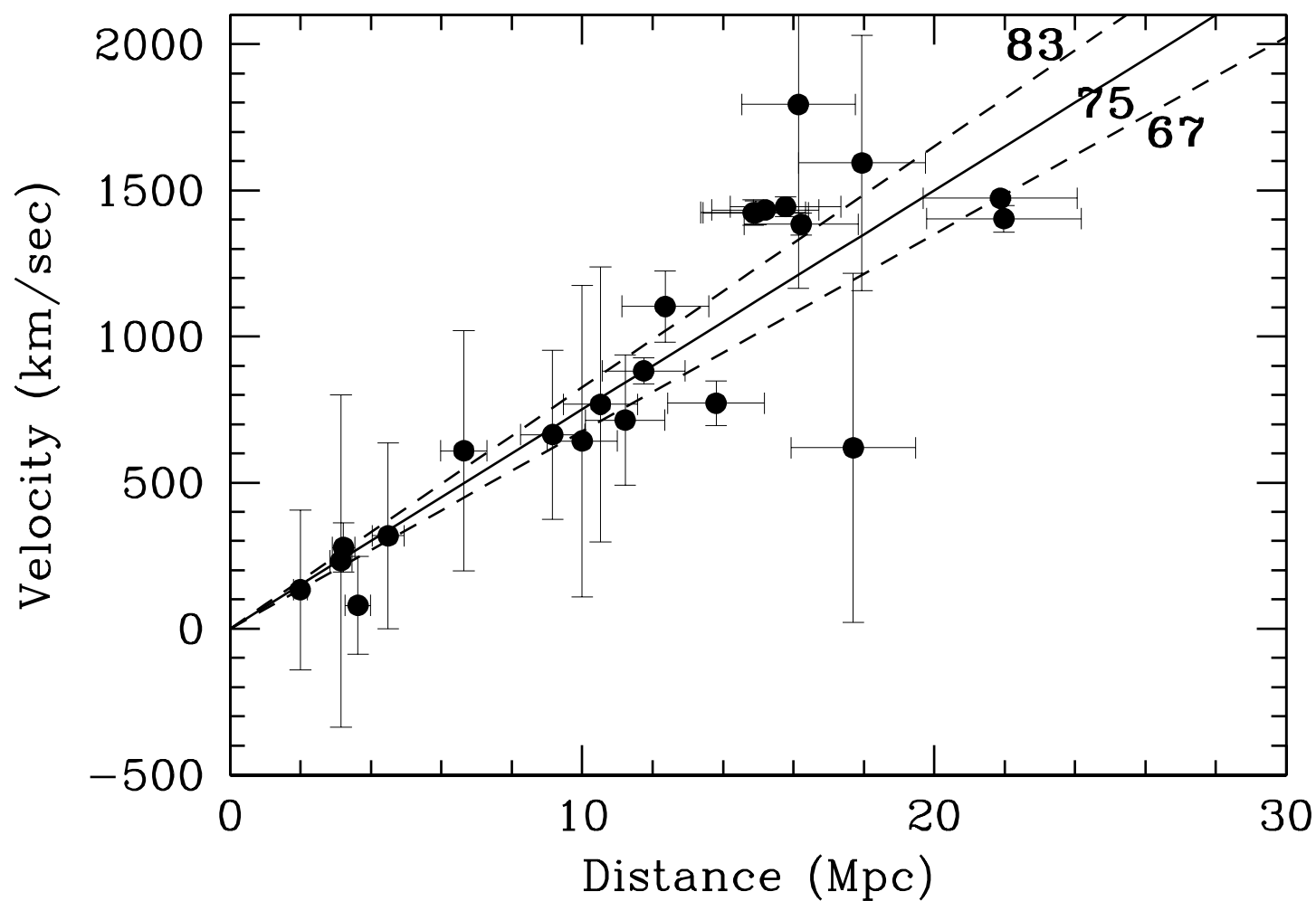
Hubble Diagram for Cepheids (flow-corrected)
