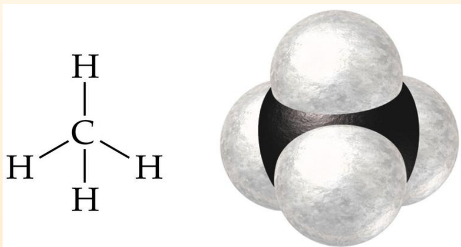
Tetrahedral geometry
