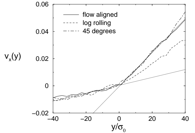
FIG. 5: Streaming velocity profiles in the flow direction, shifted such that v_x = 0 at y = 0 , at \dot{\gamma} = 0.001/\tau ( N = 115200 particles). The interface is located at y = 0 . Profiles from NI-interfaces are mirrored at y = 0 and v_x = 0 .
