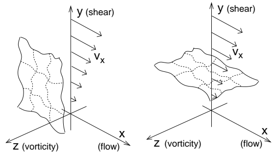
FIG. 1: Possible orientations of an interface: common strain (left) and common stress (right) geometries. Also indicated is the reference system used throughout this paper. In this paper, only the common stress case is investigated.
