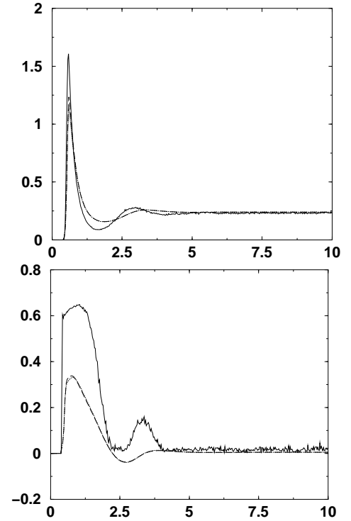
FIG. 2: (a) Density profiles for isotropic fluid with \rho^* = 0.24 and T^* = 0.5 . Solid line is the simulation data, dashed line is data obtained from DFT calculations using Eq. 4 and the Parson-Lee DCF, and the dotted line shows the density profile obtained from DFT calculations using Eq. 5 and the PL DCF. (b) Order parameter profiles for isotropic fluid with \rho^* = 0.24 and T^* = 0.5 . same symbols as in (a).
