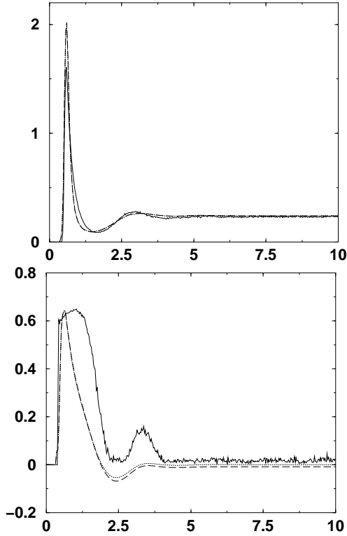
FIG. 1: (a) Density profiles for isotropic fluid with \rho^* = 0.24 and T^* = 0.5 . Solid line is the simulation data, dashed line shows the data obtained from DFT calculations using Eq. 4 and the numerical DCF, and the dotted line shows the data obtained from DFT calculations using Eq. 5 and the numerical DCF.
