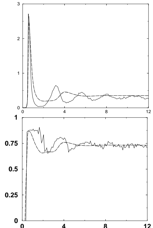
FIG. 4: (a) Density profiles for nematic fluid. Solid line is the simulation data ( \rho^* = 0.30 and T^* = 0.5 ), dashed line is data obtained from DFT calculations using Eq. 4 and Parson-Lee DCF ( \rho^* = 0.35 and T^* = 0.5 ), and the dotted line shows the data obtained from DFT calculations using Eq. 5 and Parson-Lee DCF ( \rho^* = 0.35 and T^* = 0.5 ). (b) Order parameter profiles for nematic fluid. Same symbols as in (a).
