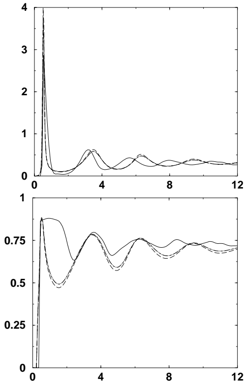
FIG. 3: (a) Density profiles for nematic fluid with \rho^* = 0.30 and T^* = 0.5 . Solid line is the simulation data, dashed line is the data obtained from DFT calculations using Eq. 4 and numerical DCF, and the dotted line shows the data obtained from DFT calculations obtained from DFT calculations using Eq. 5 and the numerical DCF. (b) Order parameter profiles for nematic fluid with \rho^* = 0.30 and T^* = 0.5 . Same symbols as in (a).
