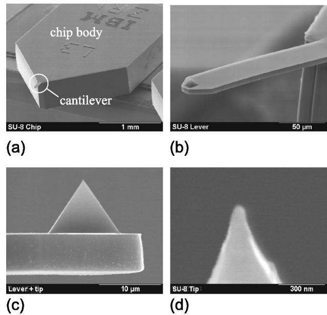
FIG. 4. (a) General view of an SU-8 SFM probe. (b) Close up of an SU-8 lever. (c) Close-up of a pyramidal tip at the end of the lever. (d) Close-up of an SU-8 tip. Radius of curvature is approximately 30 nm.
