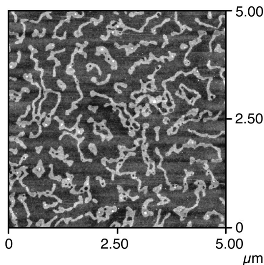
FIG. 6. AFM image ( 5 \times 5 \mu\text{m}^2 ) of a mixed Langmuir–Blodgett film with coexisting hydrocarbon and fluorocarbon molecular domains. The image z range corresponds to 5 nm (see the text for details).
