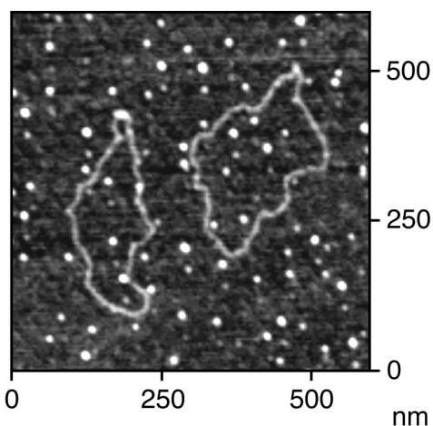
FIG. 7. AFM image ( 0.6 \times 0.6 \mu\text{m}^2 ) of DNA–plasmid (pGEM-3Zf vector from Promega Corporation, Madison, WI). The width of the DNA strand is 5–6 nm. The z scale was color adjusted to 1.5 nm.
