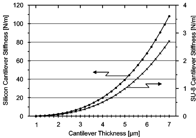
FIG. 2. Spring constant of silicon and SU-8 cantilevers as a function of thickness. Cantilevers have a length of 156 \mu\text{m} and a width of 30 \mu\text{m} .
