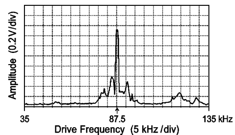
FIG. 5. Frequency response of an SU-8 cantilever. Dimensions are t=6.6 \mu\text{m} , w=31 \mu\text{m} , l=150 \mu\text{m} .
