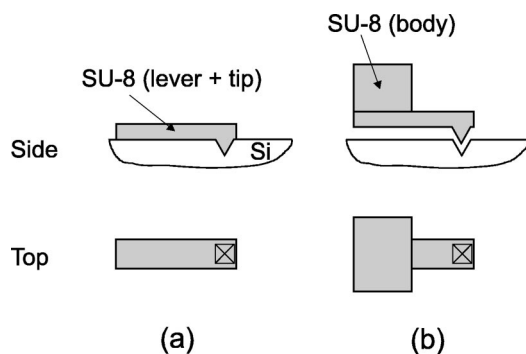
FIG. 3. (a) Formation of an SU-8 cantilever. The tip is formed by the resist molded in the pyramidal pit. (b) Free-standing cantilever is obtained upon unrolling of the chip.
