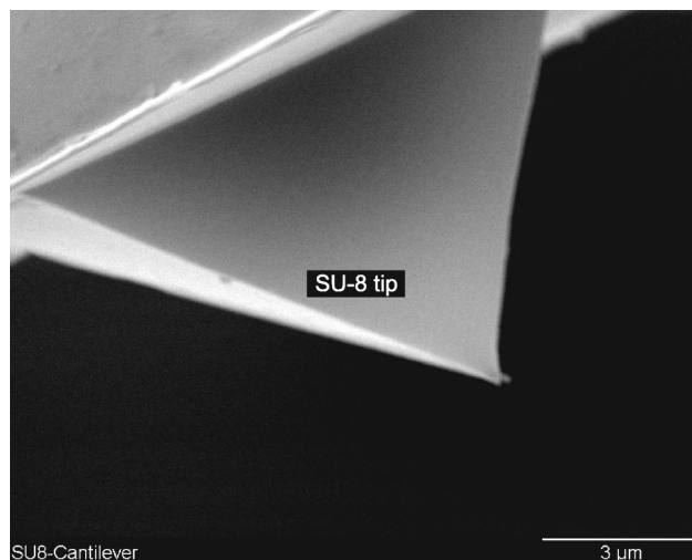
FIG. 8. SEM image of a tip after AFM imaging of soft samples. The tip showed no wear after imaging.
