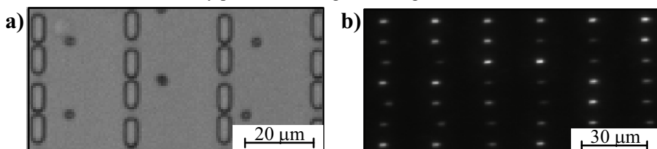
Figure 1: a) Bright field microscopy image of migrating latex particles (dark dots) in the structured ANM device with periodical obstacles (bright, rectangular) b) Fluorescence microscopy image of DNA molecules (bright spots) trapped by positive dielectrophoresis in a channel with an array of posts in an electric field of 150 V/cm of 100 Hz frequency. The non fluorescent posts are invisible in this image.
