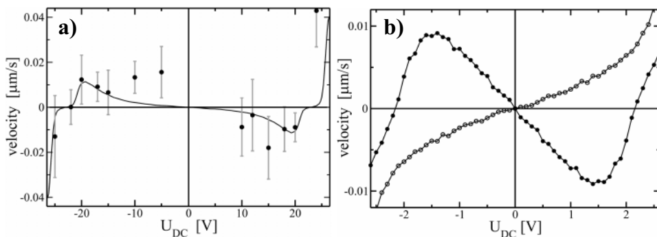
Figure 2: a) Absolute negative mobility in a microfluidic device: Dots: Experimentally obtained average velocities for 2 \mu\text{m} latex beads in a periodically arranged obstacle array subjected to a periodically switching voltage with static offset U_{DC} . Solid line: numerical simulation of particle velocities adapted to the experimental parameters. b) Numerical simulation of migration velocities as obtained for two different bead sizes. The beads with 2 \mu\text{m} diameter (dots) show ANM whereas the beads with 3 \mu\text{m} diameter (open circles) demonstrate "normal" response behaviour.
