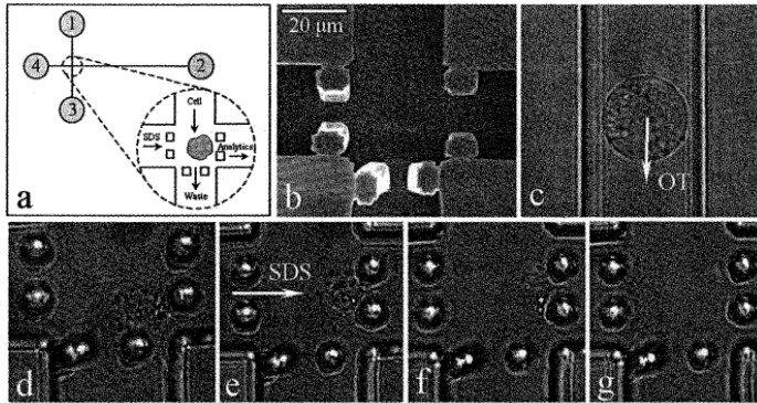
Fig. 1 (a) Scheme of our PDMS microfluidic device. Inset: channel crossing with the cell trap composed of microstructured obstacles, (b) scanning electron micrograph of the cell trap, (c) single cell in a channel navigated by OTs in the microchannel, and (d–g) optical micrographs of a single cell at the injection position during SDS lysis. SDS flow is from channel 4 through the cell trap into channel 2.
