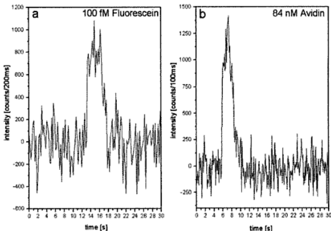
Fig. 3 (a) Electropherogram for the VIS LIF detection of 100 fM fluorescein injected into the PDMS microchannel device (separation electric field 1250 V/cm). Baseline correction and background subtraction were applied to the original data. (b) Electropherogram for the VIS LIF detection of 84 nM fluorescein-avidin injected into a PDMS device with a separation field strength of 1500 V/cm. Laser power was 25 mW for both electropherograms.
