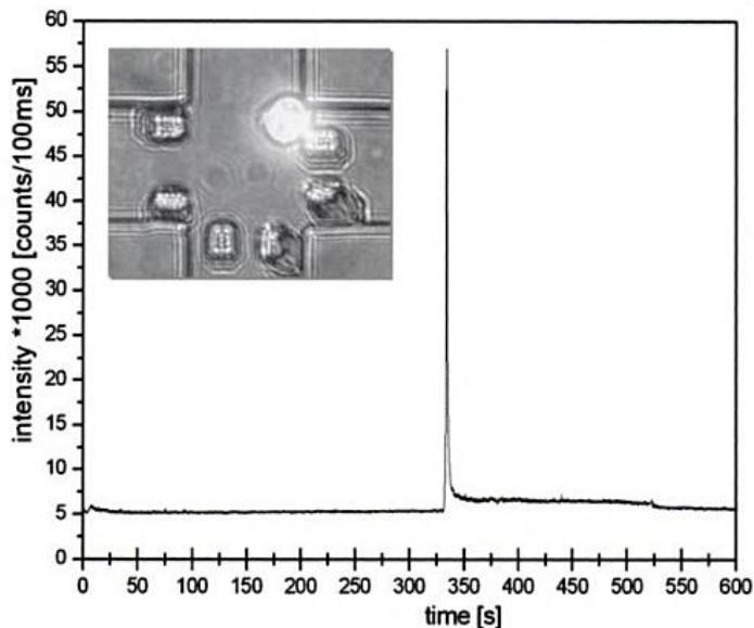
Fig. 5 Electropherogram of a single GFP-Sf9 insect cell with a distinct single component peak of the 49.5 kDa T31N-GFP variant. Starting point (0 s) of the electropherogram is defined by the application of the separation voltage to the horizontal channel and thus does not represent the initiation of cell lysis. Power of the incident laser light (at 488 nm) was 2 mW and the pinhole size 200 \mu\text{m} . Inset: Fluorescence micrograph of a single GFP-Sf9 insect cell captured at the injection position (for details see text).
