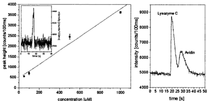
Fig. 4 Separation and detection in the UV. (a) Peak heights versus Trp concentration for injections in a PDMS microchannel: the line represents a linear regression with r = 0.998 indicating a theoretical detection limit of 17 \mu\text{M} Trp with S/N = 3 . Inset: Electropherogram of 50 \mu\text{M} injected Trp in 10 mM Tris with the detection window placed at 10 mm after the cross injector. An electrical field of 350 V/cm was used during the loading phase of the injection and of 325 V/cm during the separation phase, respectively. (b) Electropherogram for the separation of lysocyme C and avidin. Sample and running buffer was 10 mM Tris and concentrations of avidin and lysocyme C were 125 and 500 \mu\text{M} , respectively. For the injection, the analyte was loading the cross injector at 350 V/cm and a separation electrical field of 770 V/cm was used for separation. Separation length was 12 mm.
