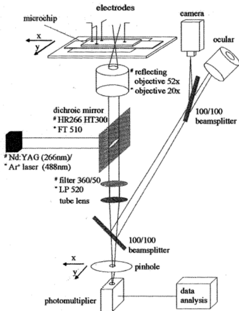
Fig. 2 Scheme of the setup for the UV (#) and VIS (*) LIF detection systems realized on an inverted optical microscope.
